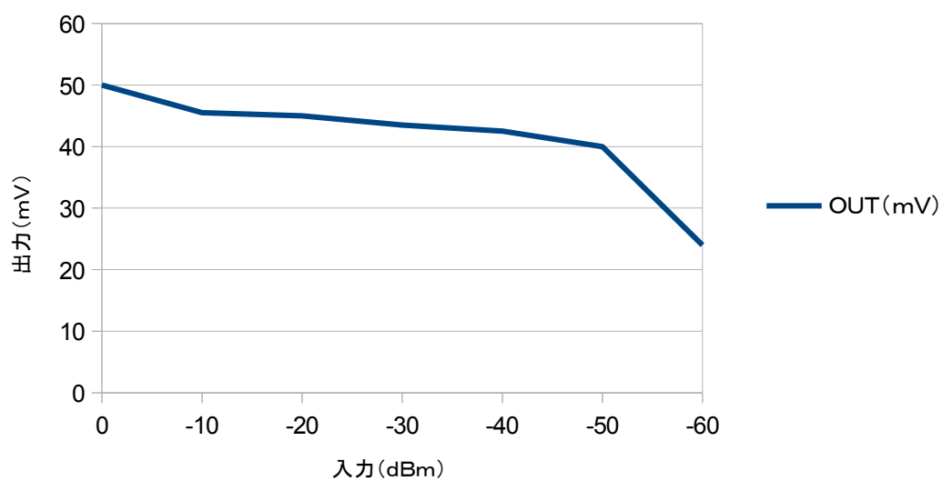
2SC2901x2 IF-Amp AGC
